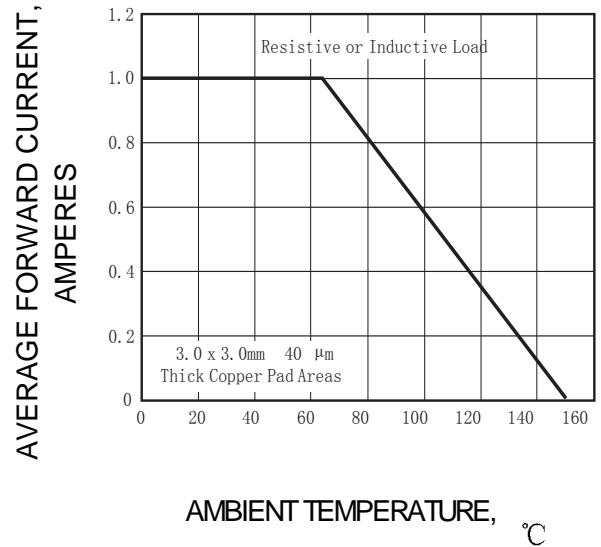
FIG.4 – FORWARD DERATING CURVE
