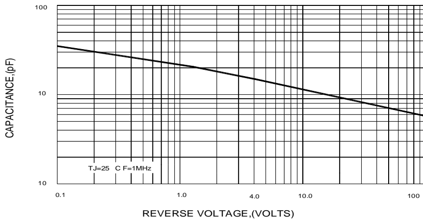
FIG.4-TYPICAL JUNCTION CAPACITANCE
